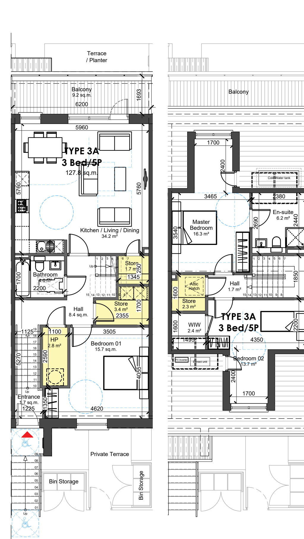
First Floor
