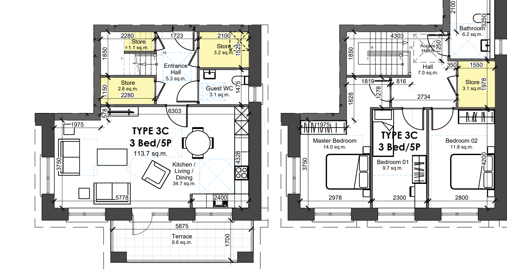
First Floor
