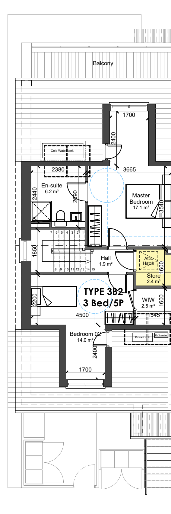
Second Floor
