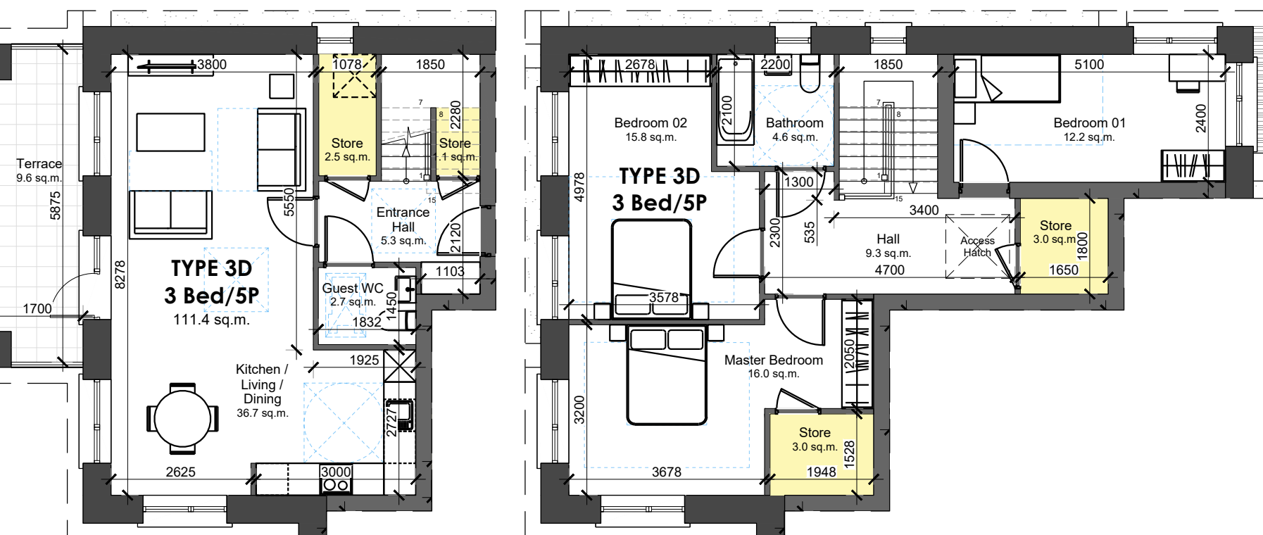
First Floor
